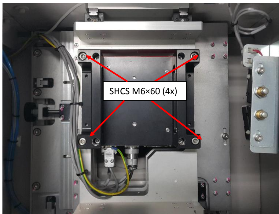
Figure 2 X-ray tube holder
