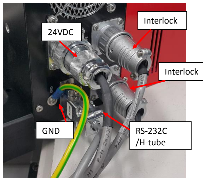
Figure 6 X-ray tube cables
